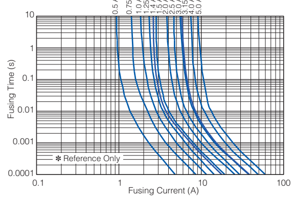
● 0603 inch / 1608 mm size (Type ERBRE)
