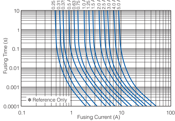
● 0402 inch / 1005 mm size (Type ERBRD)
