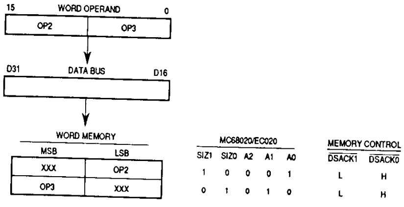
Figure 5-12. Misaligned Word Operand Write to Word Port Example
