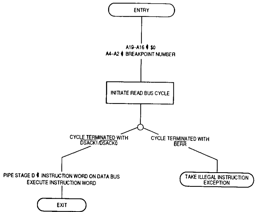
Figure 6-6. Breakpoint Instruction Flowchart
