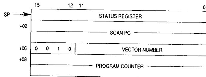
Figure 7-45. MC68020/EC020 Postinstruction Stack Frame
