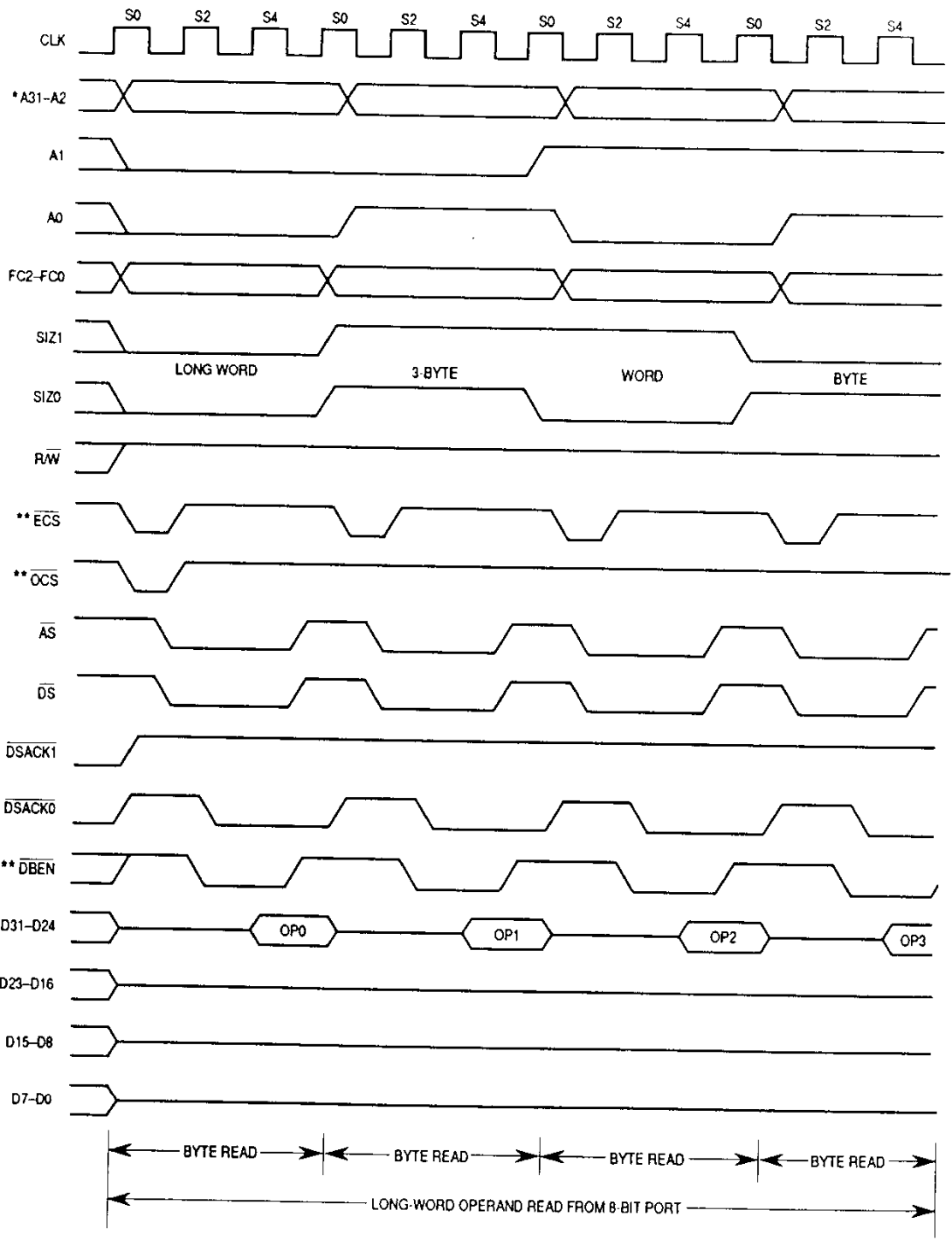
Figure 5-22. Long-Word Read—8-Bit Port
