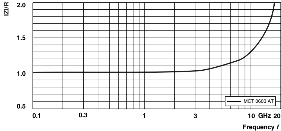
IZI/R for 49.9 \Omega chip resistor
